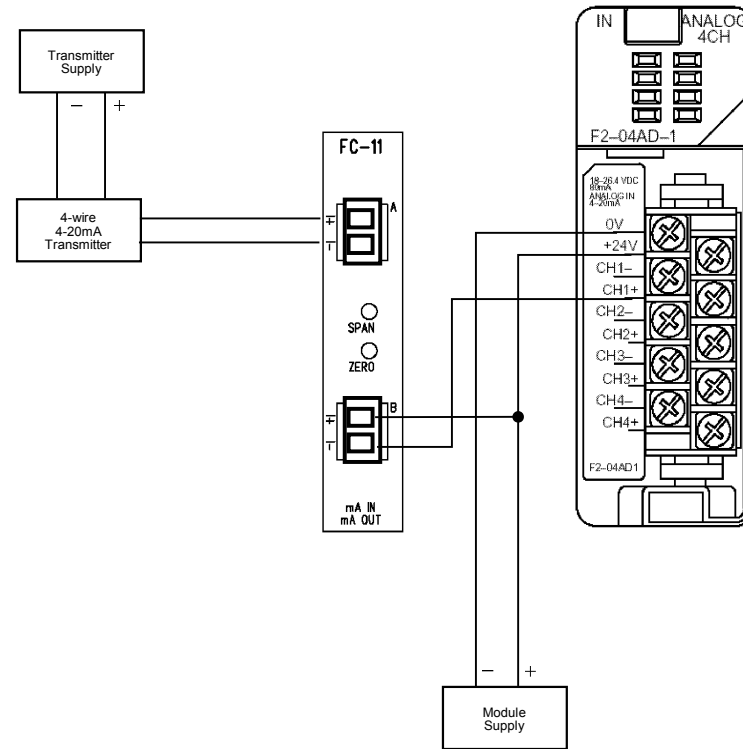
4-Wire Transmitter, 4-20 mA Input to 4-20 mA Sinking Input (example)
